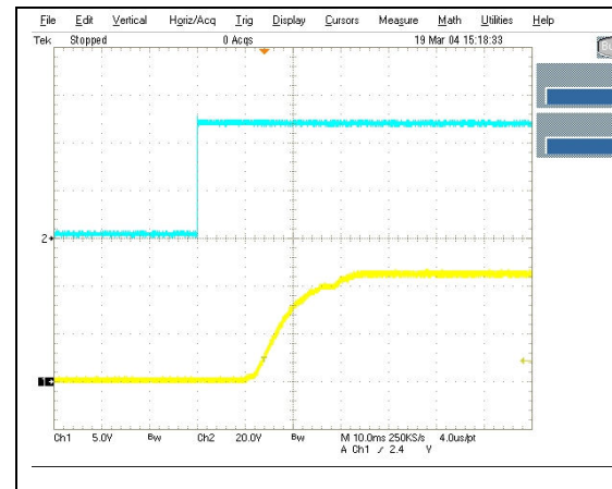
iEB48013A120V-000 Typical startup characteristic from input voltage application at full load, 10mS/div. Upper trace - input voltage 20V/div, lower trace – output voltage 5V/div
