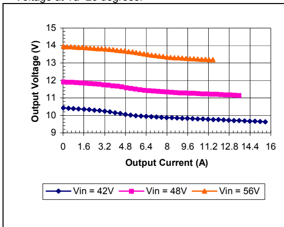
iEB48013A120V-000 Typical Output Voltage vs. Load Current at Ta = 25 degrees
