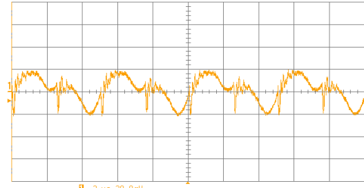
iEB48013A120V-000 Typical Output Ripple at nominal Input voltage and full load at Ta=25 degrees pkpk(1) average low high sigma 41.4mV 10.92mV 38.8 43.1 0.7 rms(1) 10.92mV 10.51 11.58 0.16 STOPPED
