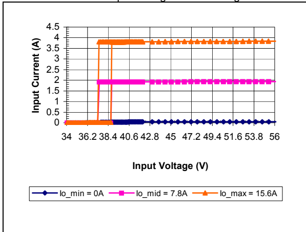
iEB48013A120V-000 Typical Input Current vs. Input Voltage Characteristics
