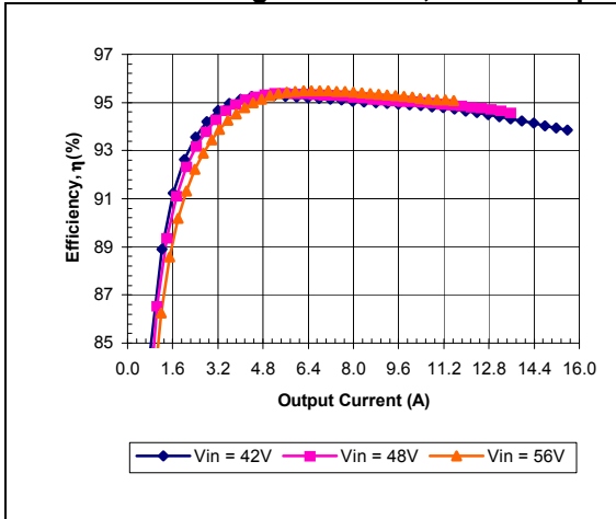
iEB48013A120V-000 Typical Efficiency vs. Input Voltage at Ta=25 degrees.
