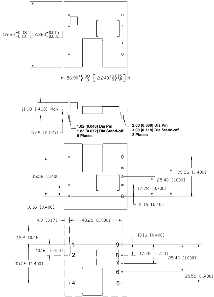
Recommended hole pattern (top view)
