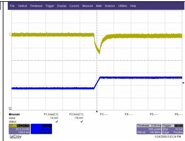
Transient Response. Load Step from 50% to 75% of Full Load with di/dt= 0.1A/uS. Ch. 1: Vo Ch. 3: Io
