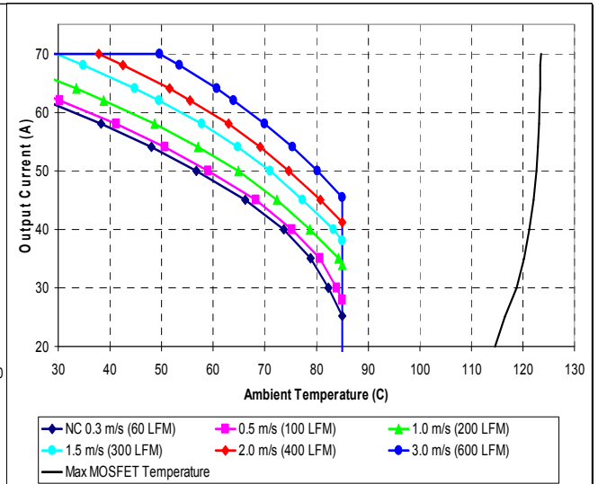
Maximum output current vs. ambient temperature at nominal input voltage for airflow rates natural convection (0.3m/s) to 3.0m/s with airflow from pin 1 to pin 4.
