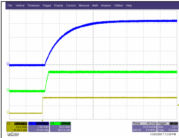
Start-up from on/off Switch at 48V input and Full Load. Ch. 1: ON/OFF Ch. 3: Vo Ch. 4: Io
