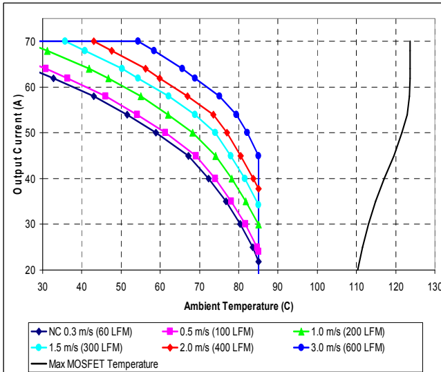
Maximum output current vs. ambient temperature at nominal input voltage for airflow rates natural convection (0.3m/s) to 3.0m/s with airflow from pin 4 to 1.
