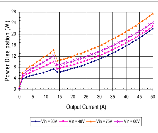
Power Dissipation vs. Input Voltage at Ta=25C
