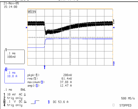
Load Transient Response. Load Step from 50% to 75% of Full Load with di/dt= 1A/uS. Ch. 1: Vo Ch. 3: Io
