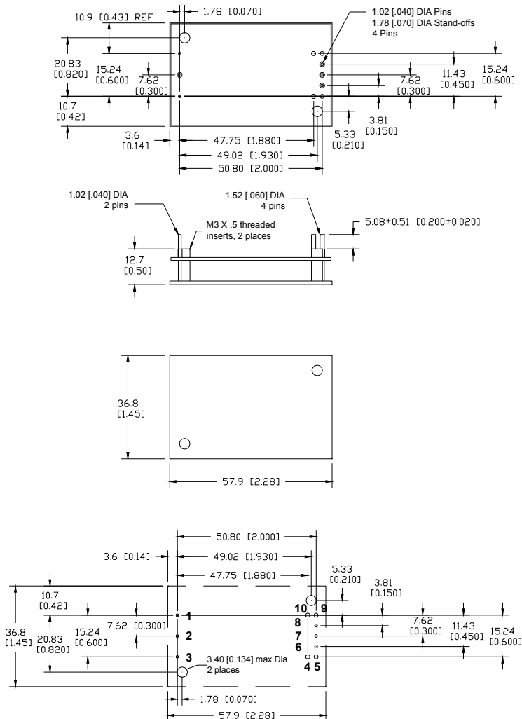
Recommended hole pattern (top view)
