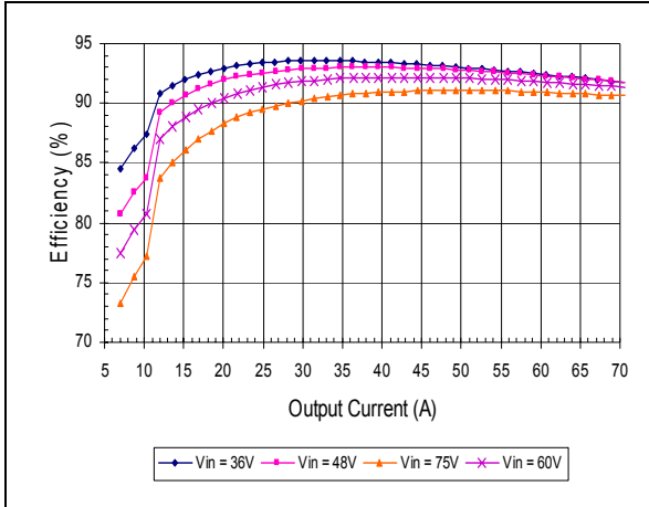
Efficiency vs. Vin at 25C (test in socket, no heat sink)
