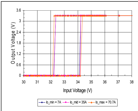
Typical Output Voltage vs. Input Turn-on and Turn-off Voltage at Ta=25C
