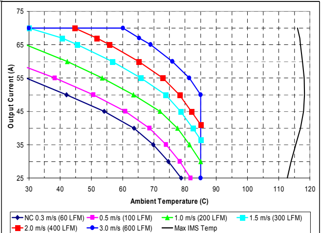
Maximum output current vs. ambient temperature at nominal input voltage for airflow rates natural convection (0.3m/s) to 3.0m/s with airflow from pin 1 to pin 3 (best orientation).
