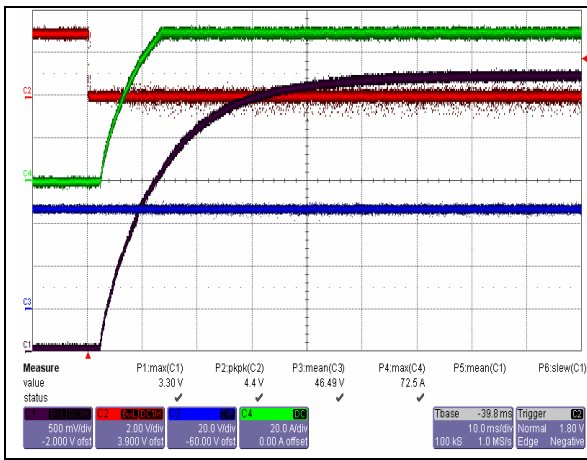
Start-up from on/off Switch at 48V input and Full Load. Ch. 1: Vo Ch. 2: ON/OFF Ch. 3: Vin Ch. 4: Io
