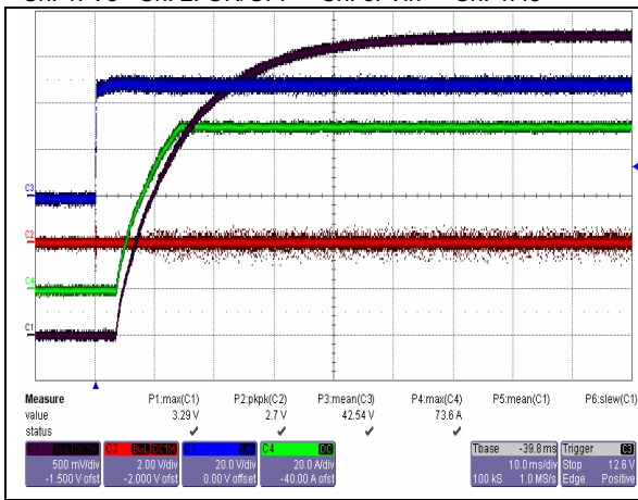
Start-up from Input Voltage Application at Full Load. Ch. 1: Vo Ch. 2: ON/OFF Ch. 3: Vin Ch. 4: Io
