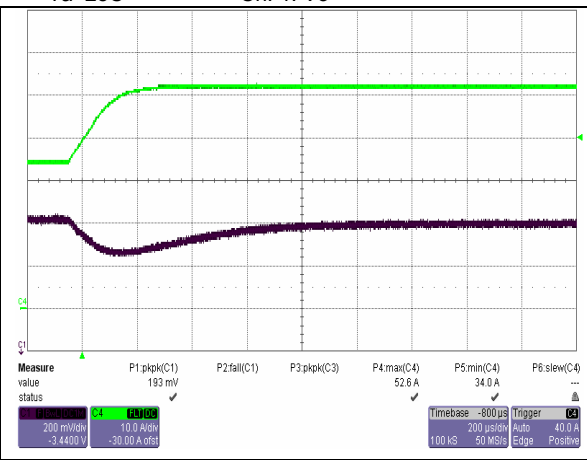
Load Transient Response. Load Step from 50% to 75% of Full Load. Ch. 1: Vo Ch. 3: Io
