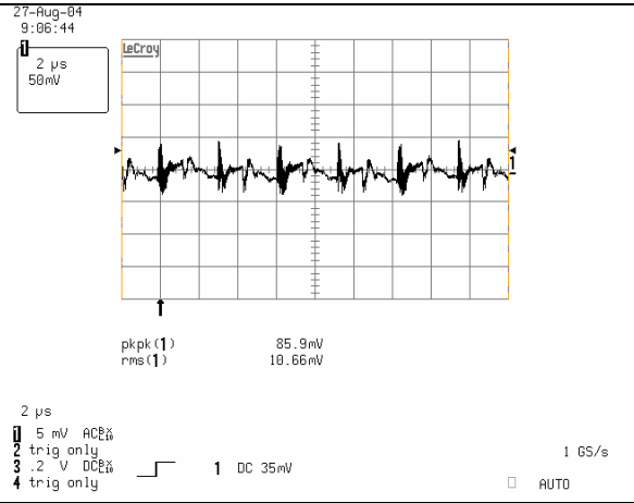
Typical Output Ripple at 48V Input and Full Load. Cext=68uF. Ch. 1: Vo
