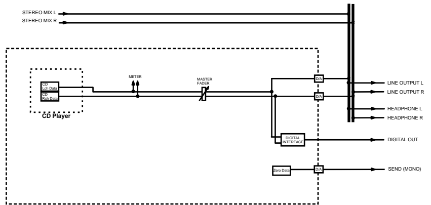
Block Diagram (CD player mode) [DP-01FX/CD only]
