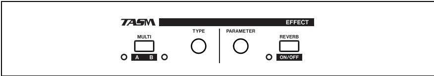
Figure 3.1: Effect controls
