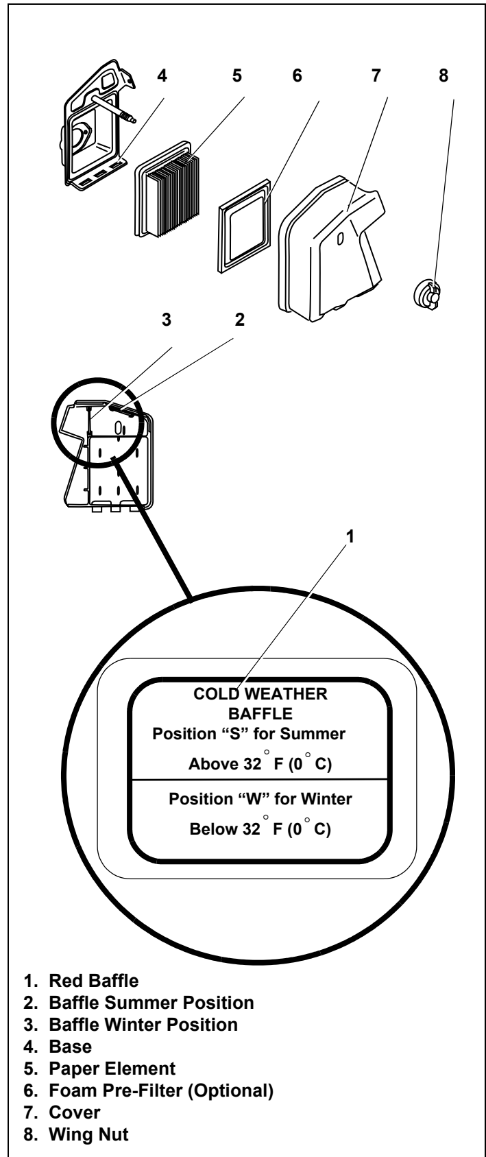
Figure 45. Type “D” Climate Guard Air Cleaner Assembly
