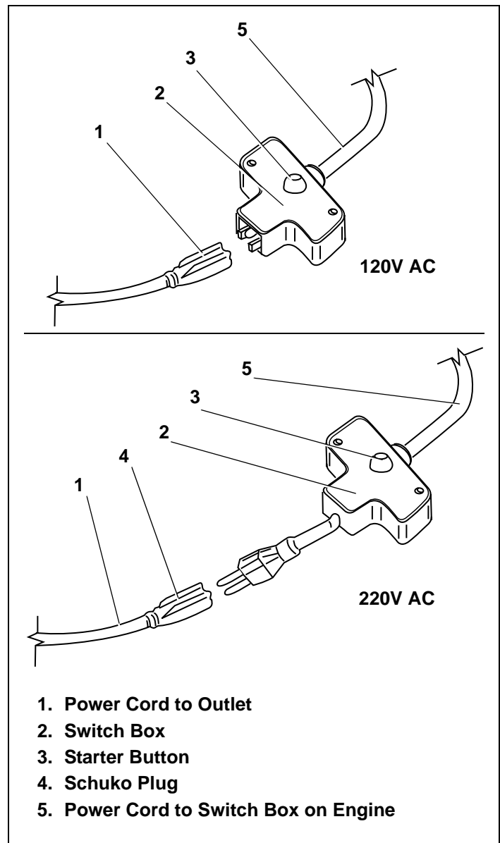
Figure 8. Electrical Applications
