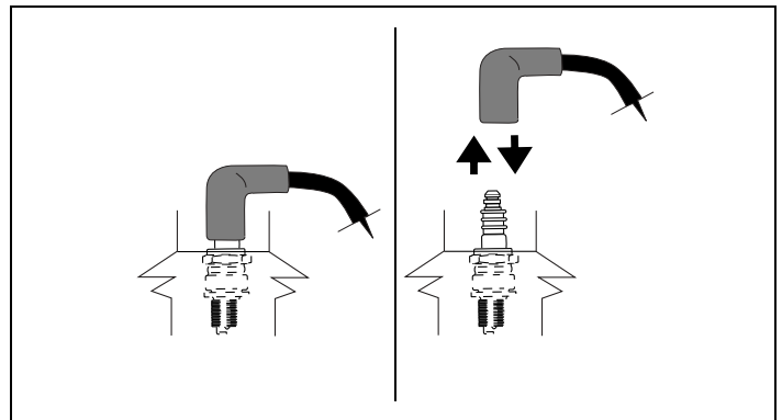
Figure 2. Disconnecting/Connecting Spark Plug
