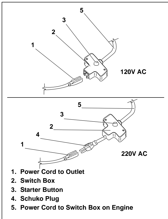
Figure 18. Electrical Applications
