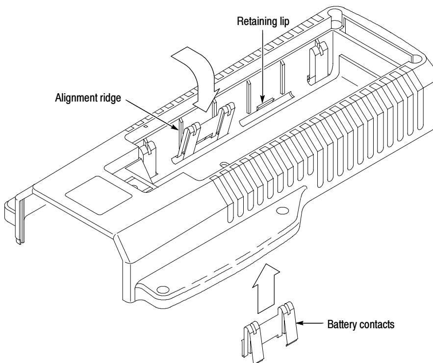
Figure 6- 15: Battery contact installation alignment
