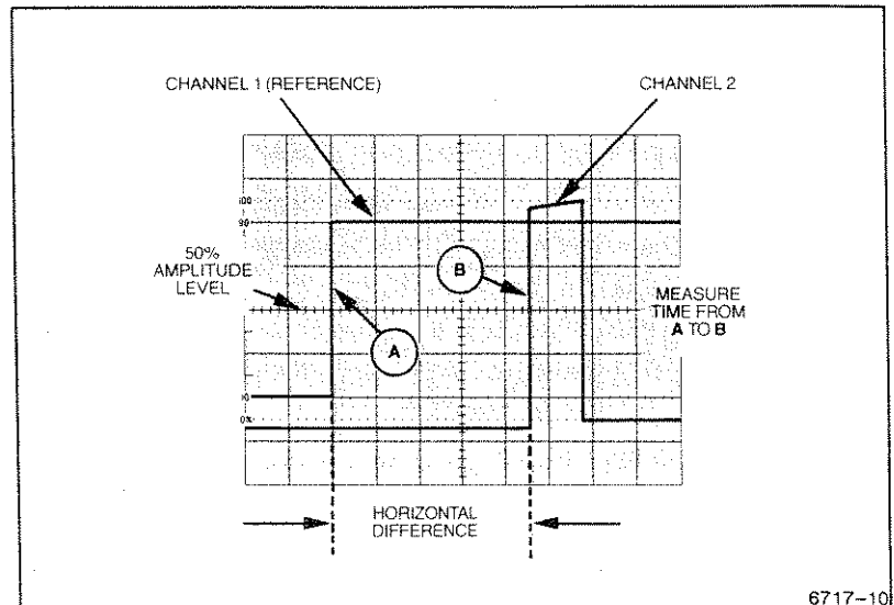
Figure 3-7. Time difference between pulses on time-related signals.
