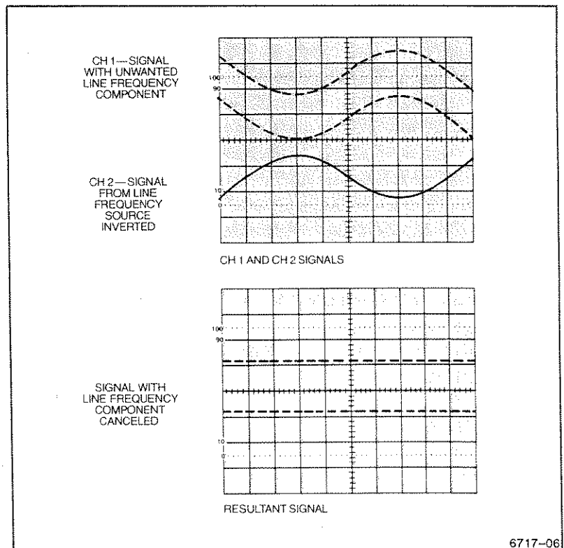
Figure 3-3. Common-mode rejection.
