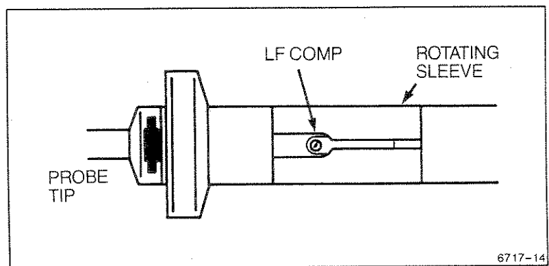
Figure 4-2. Locating the low-frequency compensation adjustment.
