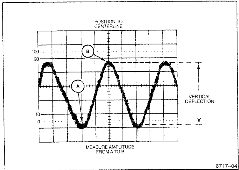
Figure 3-1. Measuring peak-to-peak voltage of a waveform.
