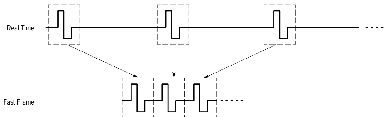
Figure 3–30: Fast Frame
