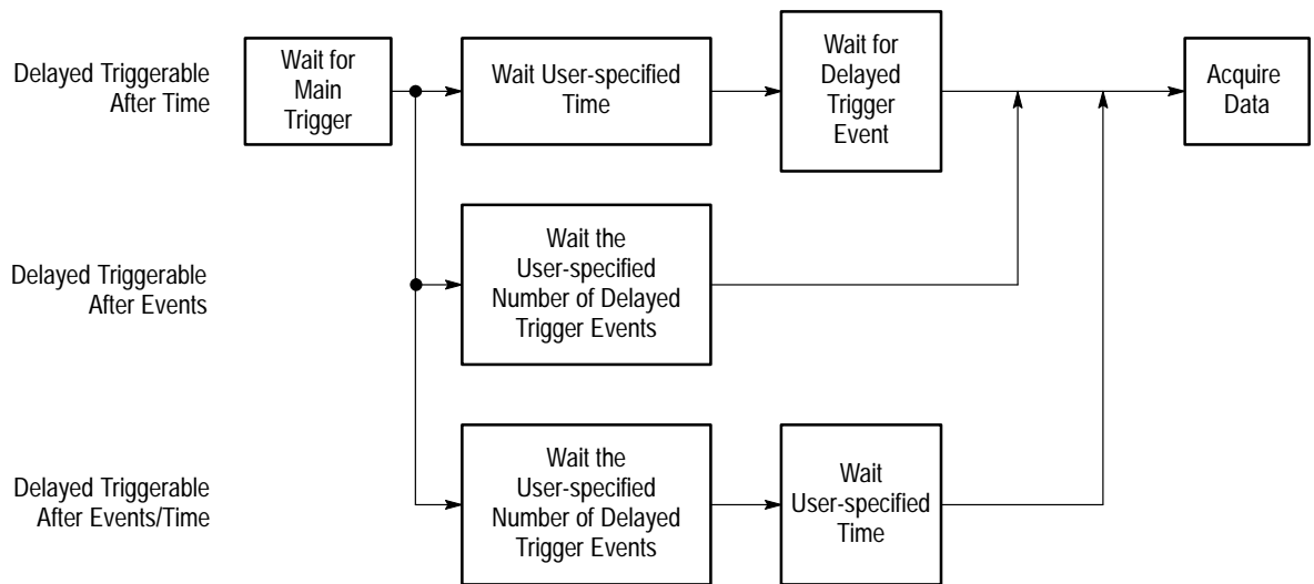
Figure 3–51: Delayed Triggerable
