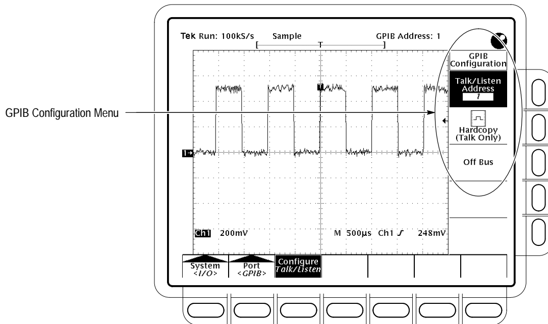
Figure 3–84: Utility Menu
