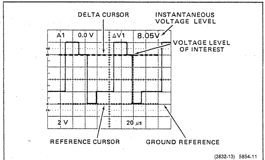
Figure 3-1. Instantaneous voltages.
