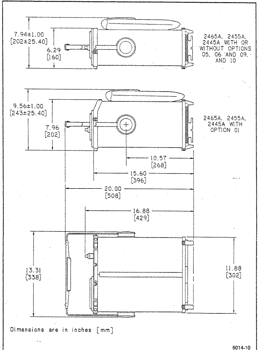
Figure 6-1. Dimensional drawing.
