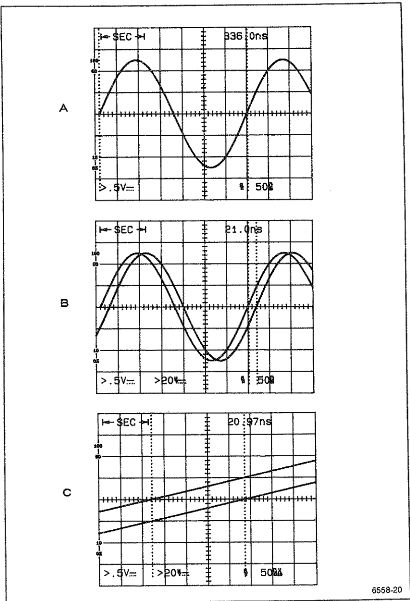
Figure 5-5. Phase difference measurement.
