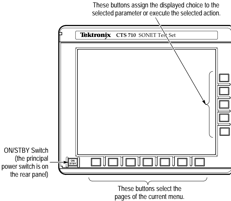
Figure 2-1: Controls Located Around the Display
