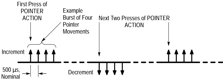
Figure 3-49: Alternating Burst Pointer Movement
