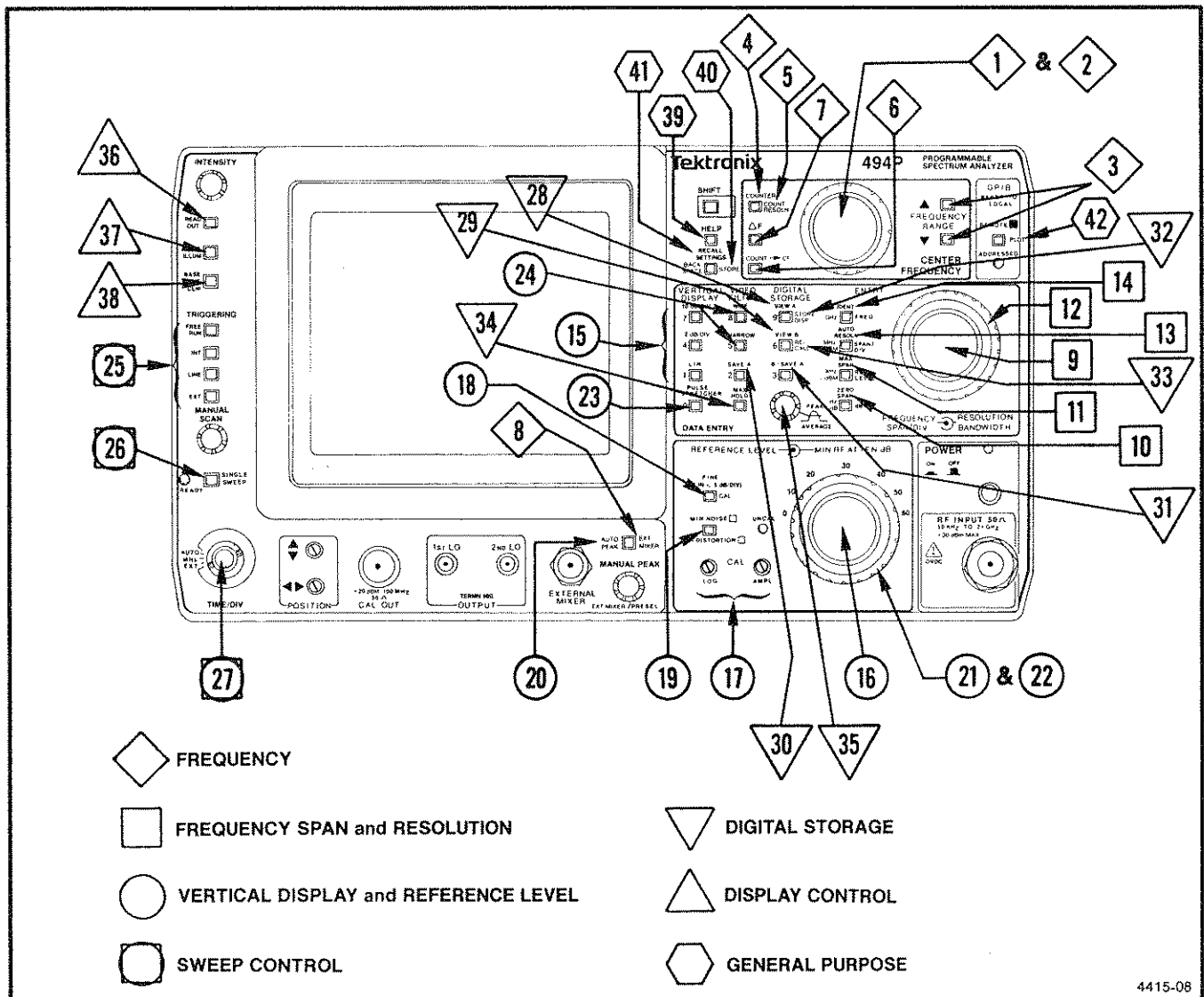
Figure 4-1. Front-panel control commands and queries.
