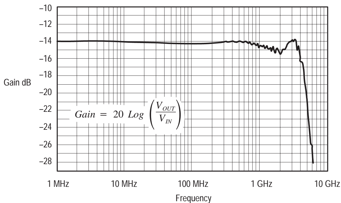
Figure 9: Typical bandwidth
