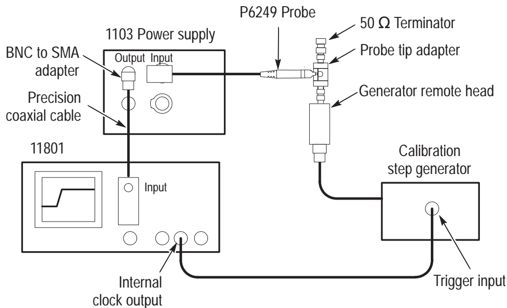
Figure 14: Test system and probe rise time setup
