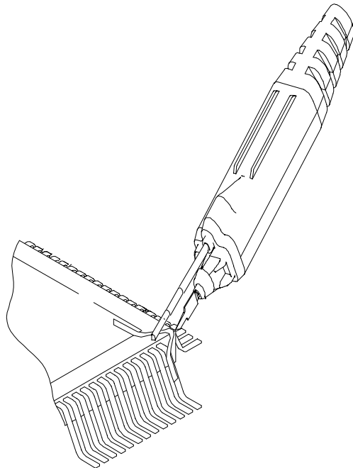
Figure 8: Low-inductance grounding
