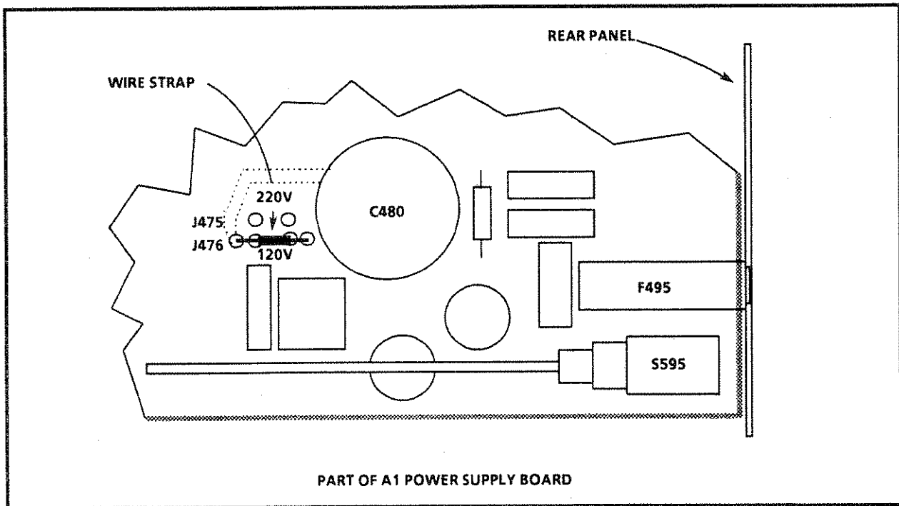
Fig. 3-2. Strap across J476 sets mains voltage to 120 V.
