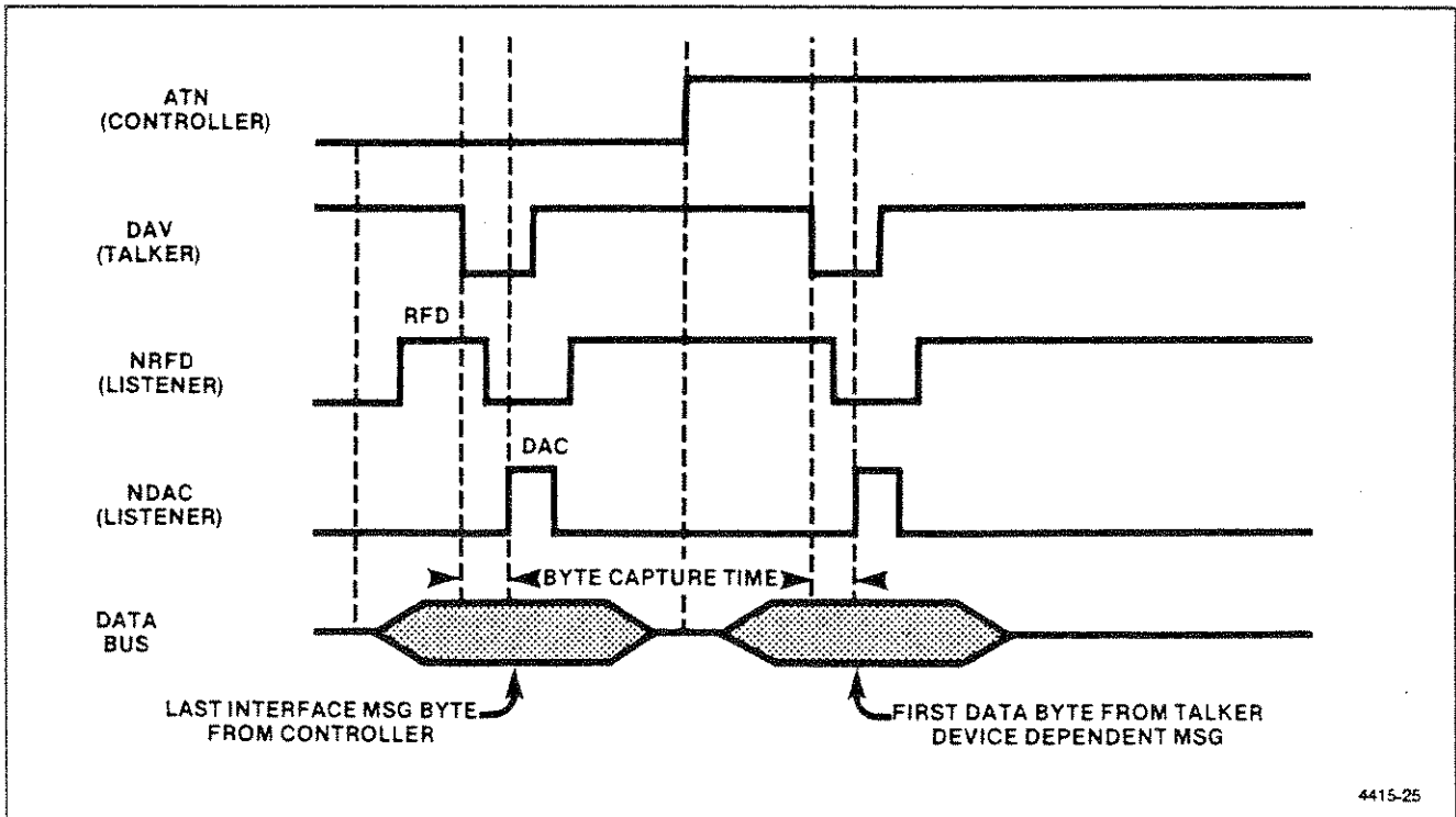
Figure A-5. A typical handshake timing sequence (idealized). Byte capture time is dependent on the slowest instrument involved in the handshake. RFD means Ready For DATA; DAC means Data Accepted.
