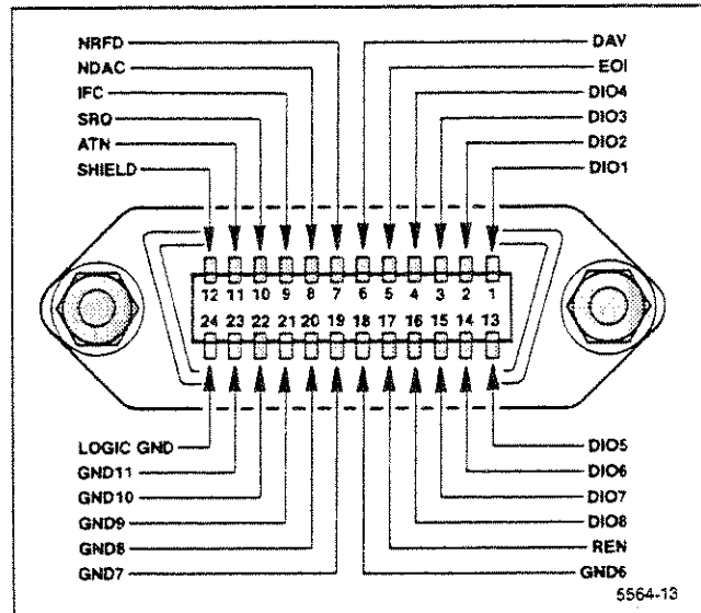
Figure A-1. IEEE Std 488 (GPIB) connector.
