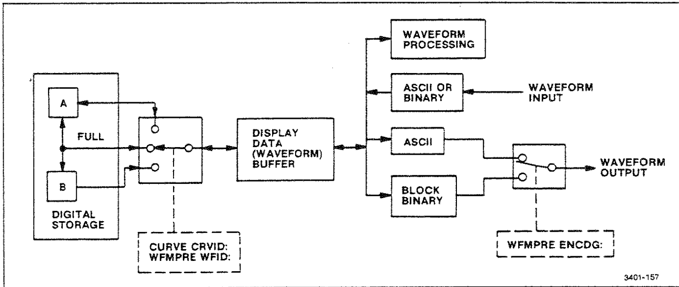
Figure 9-2. How multiple use of the display data buffer is controlled.
