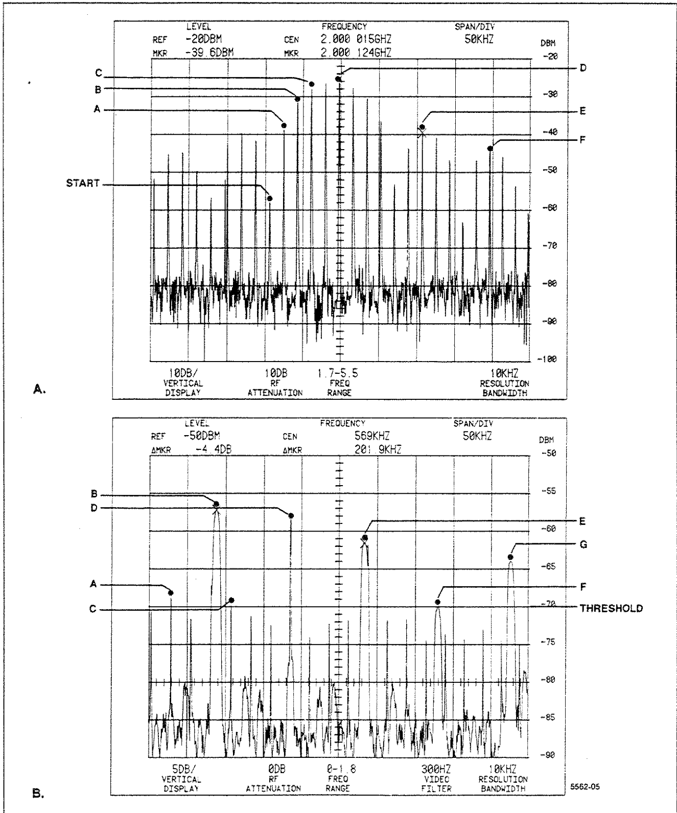
Figure 5-4. Signal finding examples.
