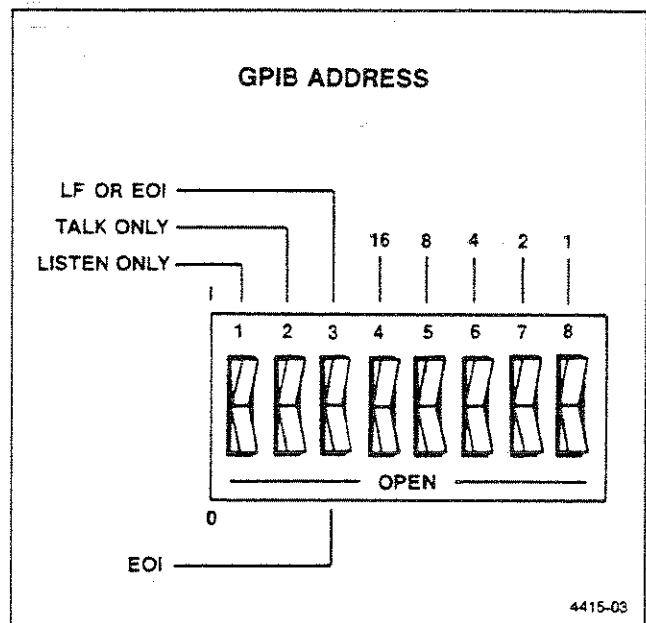
Figure 1-3. Rear-panel GPIB ADDRESS switches. The LF OR EOI switch (message terminator) and the TALK ONLY and LISTEN ONLY switches are part of the same switch band.
