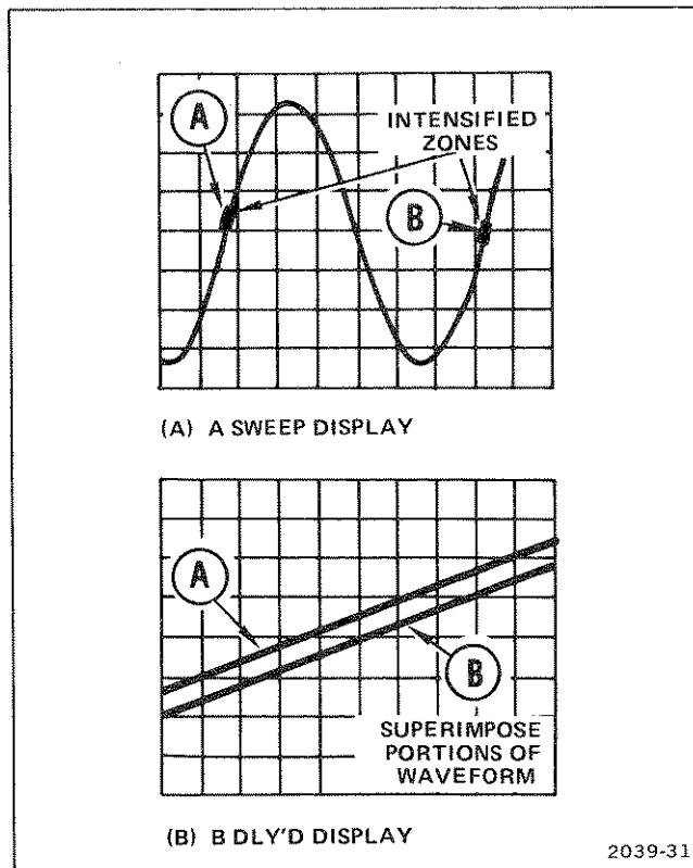
Fig. 30. Time duration and frequency measurements.
