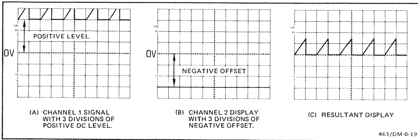
Fig. 16. Algebraic addition.
