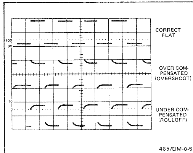
Fig. 11. Probe compensation.
