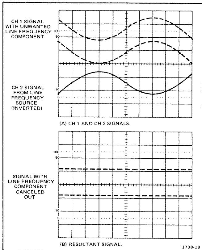
Fig. 17. Common-mode rejection.
