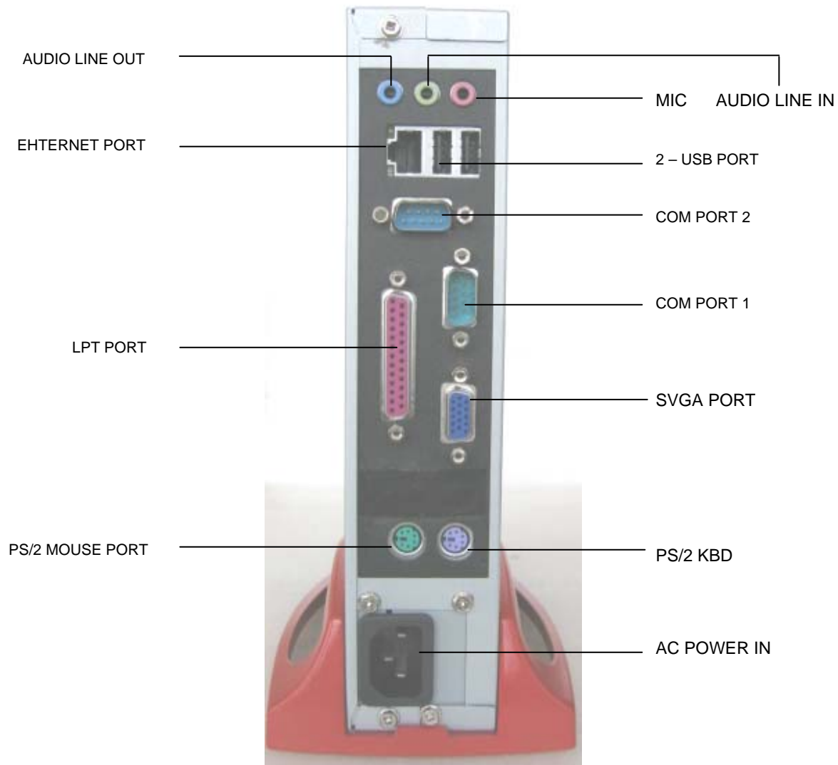
Itona TC4xyy Rear view
