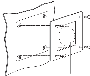
Aperture (70 mm dia.) for cable and bearing hub.
