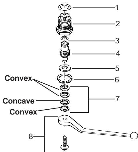
Figure 28 - Dump Valve Cartridge
