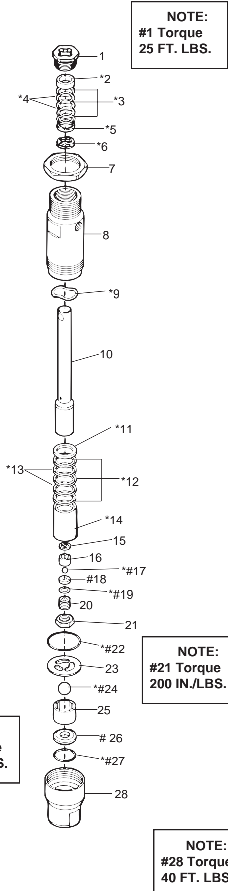
Figure 21 - Fluid Section
