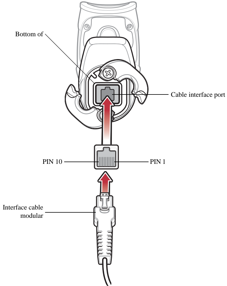
Figure 3-1. Scanner Cable Pinouts
