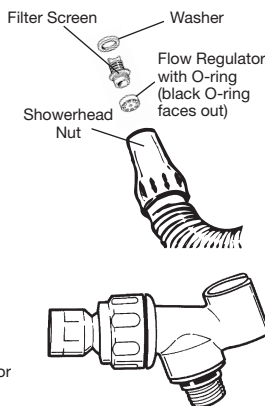
Flow Regulator
