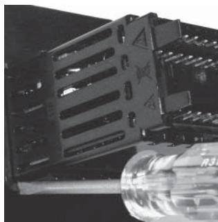
Place the blade of a screwdriver in the notch of the mounting collar assembly.
