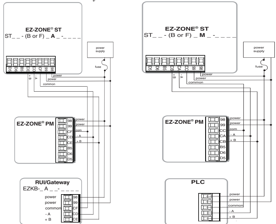
A network using Watlow's Standard Bus and an RUI/Gateway.
