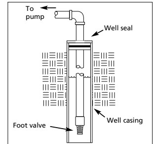
Figure 10 - Well Seal
