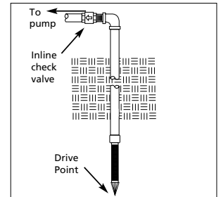
Figure 9 - In-Line Check Valve
