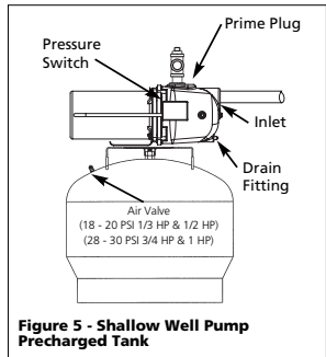
Figure 5 - Shallow Well Pump Precharged Tank
