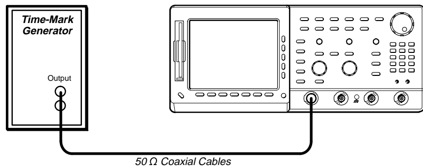
Figure 1-12: Initial Test Hookup
