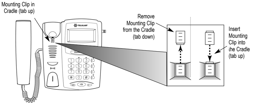
Figure 12 – Handset mounting clip for wall-mount.
