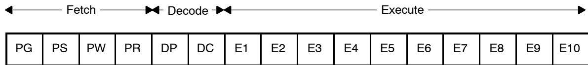
Figure 4–5. Pipeline Phases
