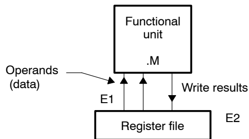
Figure 4–11. Multiply Instruction Execution Block Diagram
