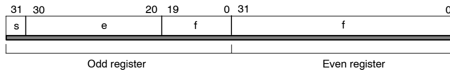
Figure 3–2. Double-Precision Floating-Point Fields
