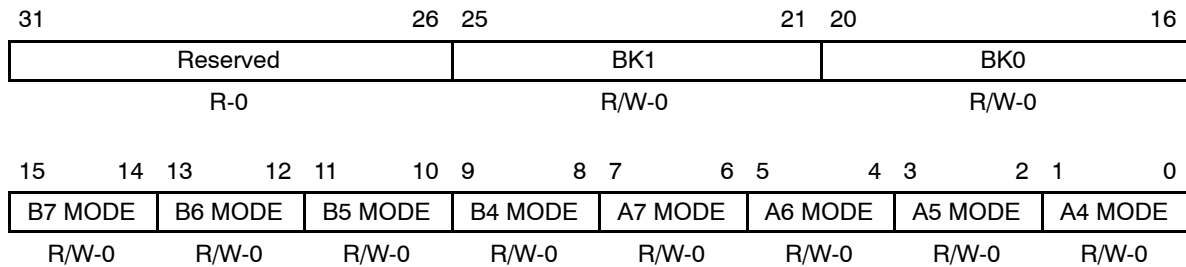
Figure 2–3. Addressing Mode Register (AMR)
