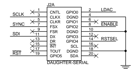
J2A (TOP) = SAM_TSM-110-01-L-DV-P J2B (BOTTOM) = SAM_SSW-110-22-F-D-VS-K
