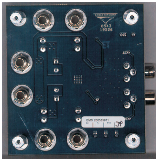
Figure 2. TI TPA3100D2 Audio Power Amplifier EVM – Bottom View
