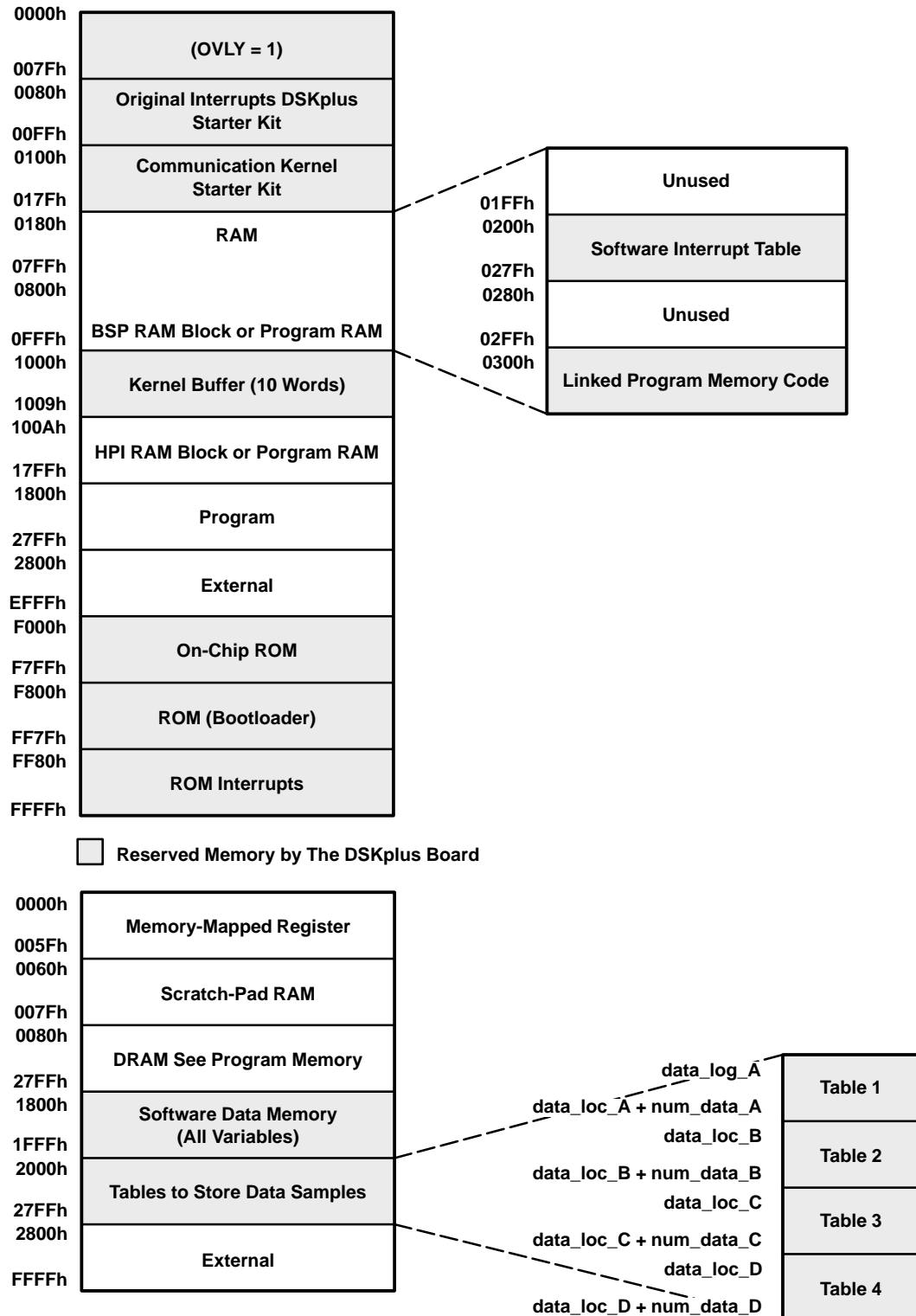
Figure 5. Memory Map
