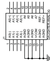
J1 (TOP) = SAMTEC - P/N: TSM-100-1-L-DV-P J1 (BOTTOM) = SAMTEC - P/N: SSW-102ZF-D-VS
