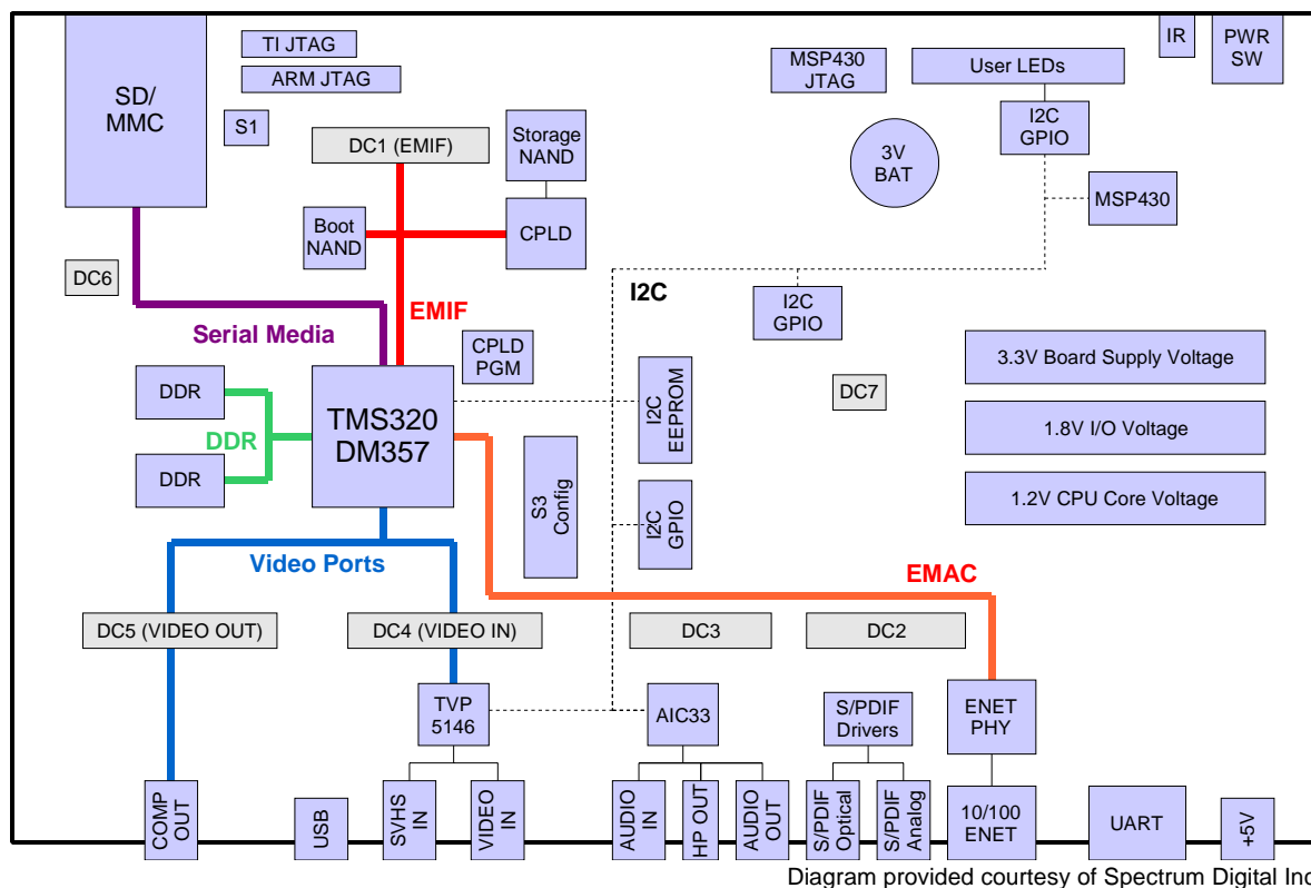
Figure 1–1 DM357 Hardware Block Diagram
