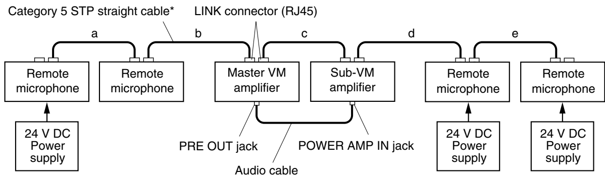
Connection example 2
