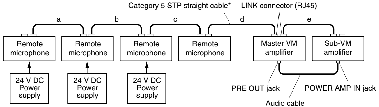
Connection example 1
