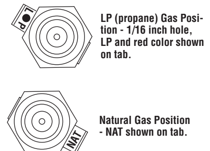
Top View of Hex Fitting and Orifice Strip Tab Figure 62
