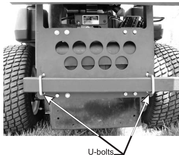
Figure 3 Outer Engine Mount Tube Attachment
