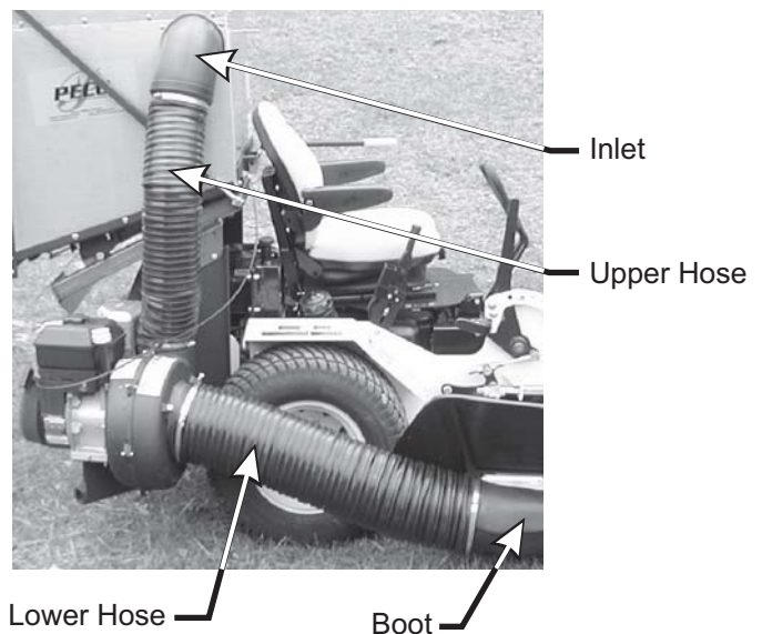
Figure 12 Hose Assembly
