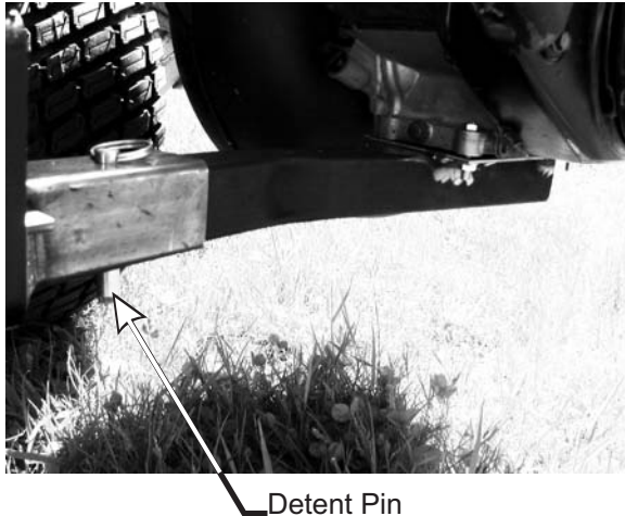
Figure 10 Engine Mount Arm
