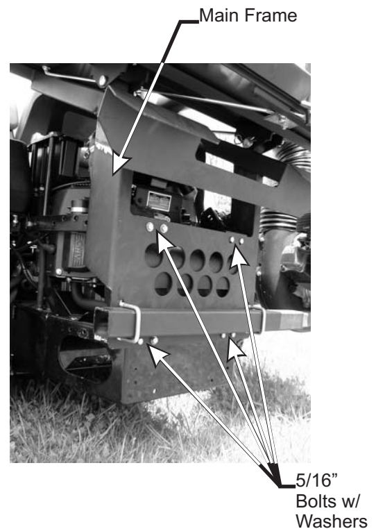
Figure 2 Main Frame Assy.
