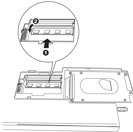
Installing the memory module
