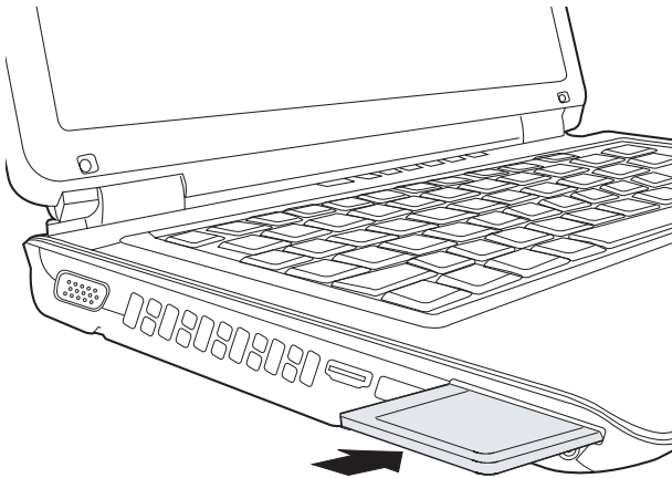
Inserting the ExpressCard
