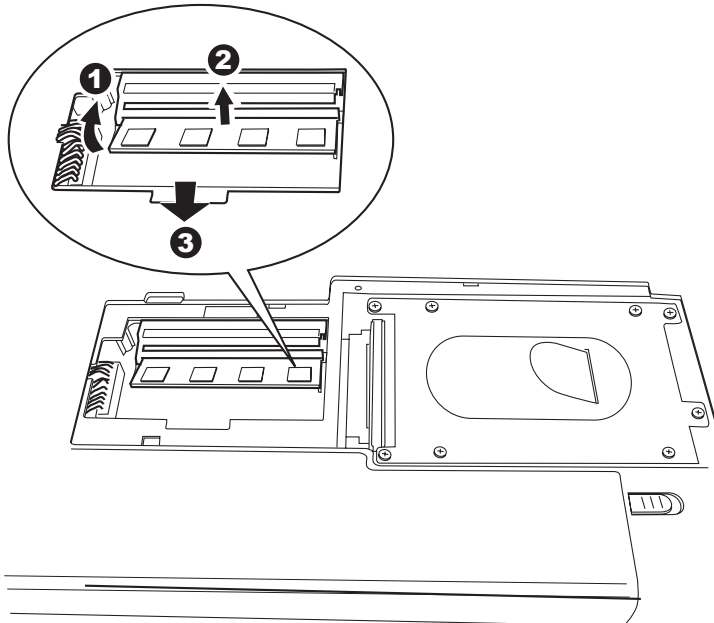
Removing the memory module
