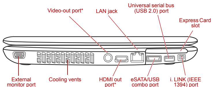
Figure 2-2 The left side of the computer
