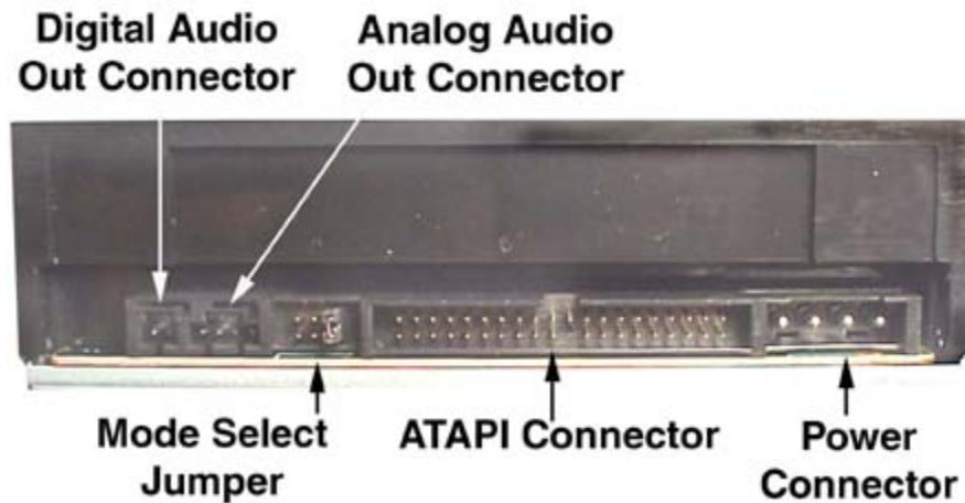
Figure 1. SD-R5372 DVD Rewritable Drive Rear Panel - Connectors
