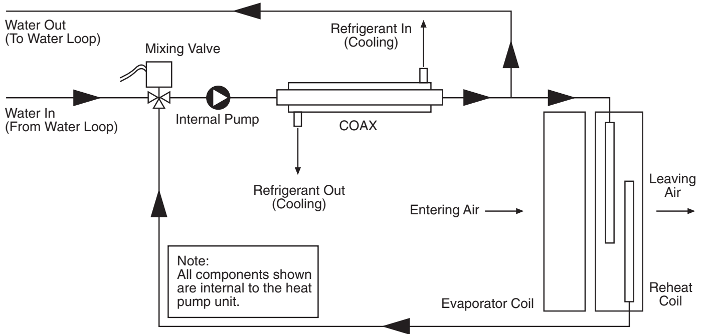
Figure 2: ClimaDry Schematic
