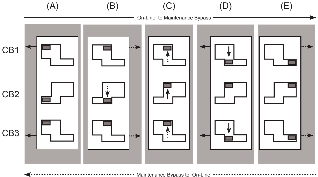
Figure 12-8 - MBS Mechanical Interlock Plate Operation
