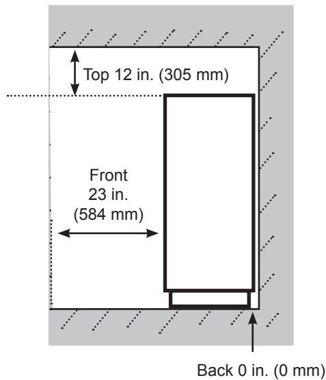
FIGURE 8.1 - UPS CLEARANCE
