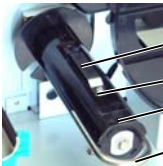
Holder Stopper B-3x4 Screw Take-up Spool Take-up Clip
