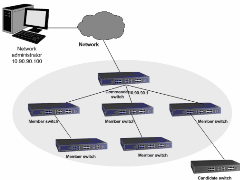
Figure 15-1 Cluster topology
