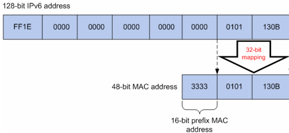
Figure 9-3 Mapping relationship between multicast IPv6 address and multicast IPv6 MAC address
