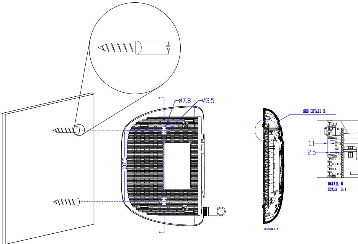
Figure 2-3 Wall-mount Install
