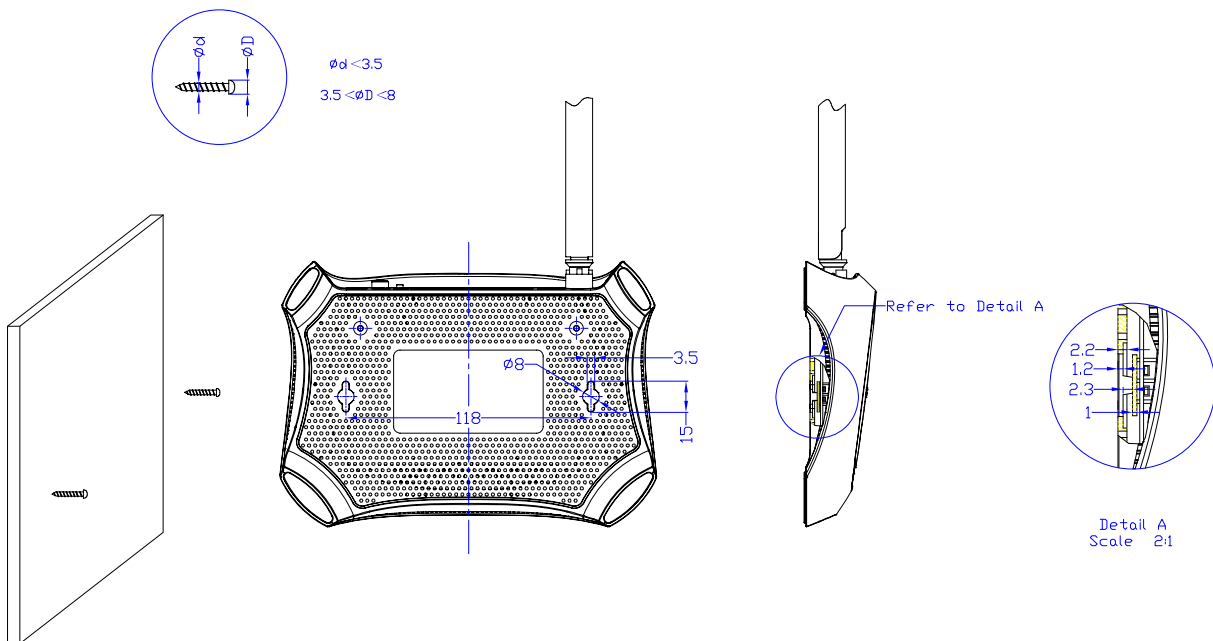
Figure 2-3 Wall-mount Install
