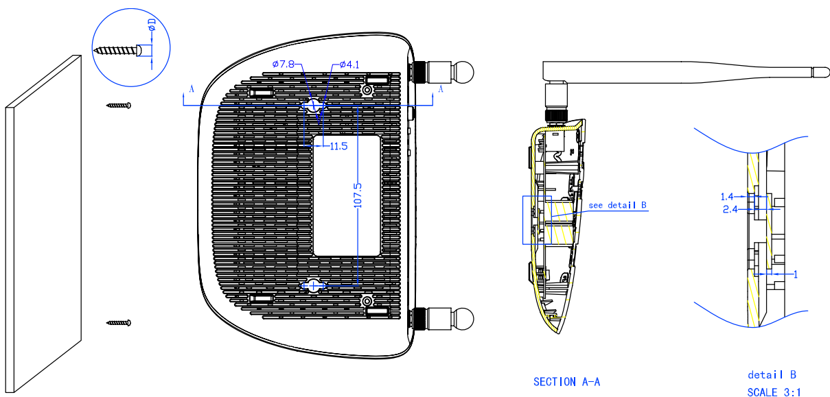
Figure 2-3 Wall-mount Install
