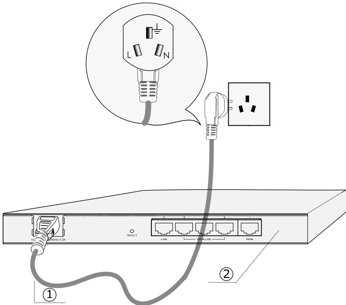
① AC Power Cord (with PE cable) ② Router (Rear Panel)
