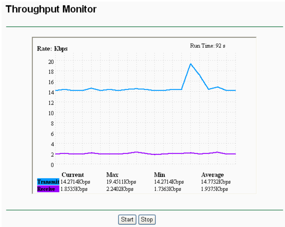
Figure 5-17 Wireless Throughput
